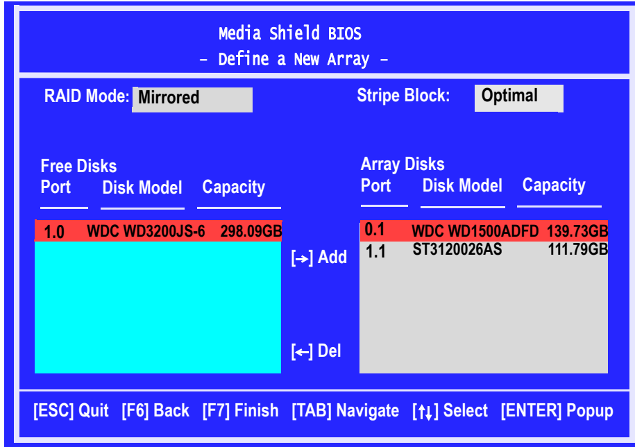
Figure 2.8 MediaShield Utility—Array Disks Assigned
